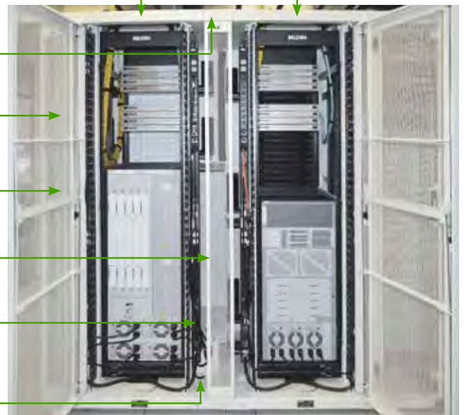
Ganged XN frames with end-of-row 6" extension and between cabinet 6" extension (rear view)
