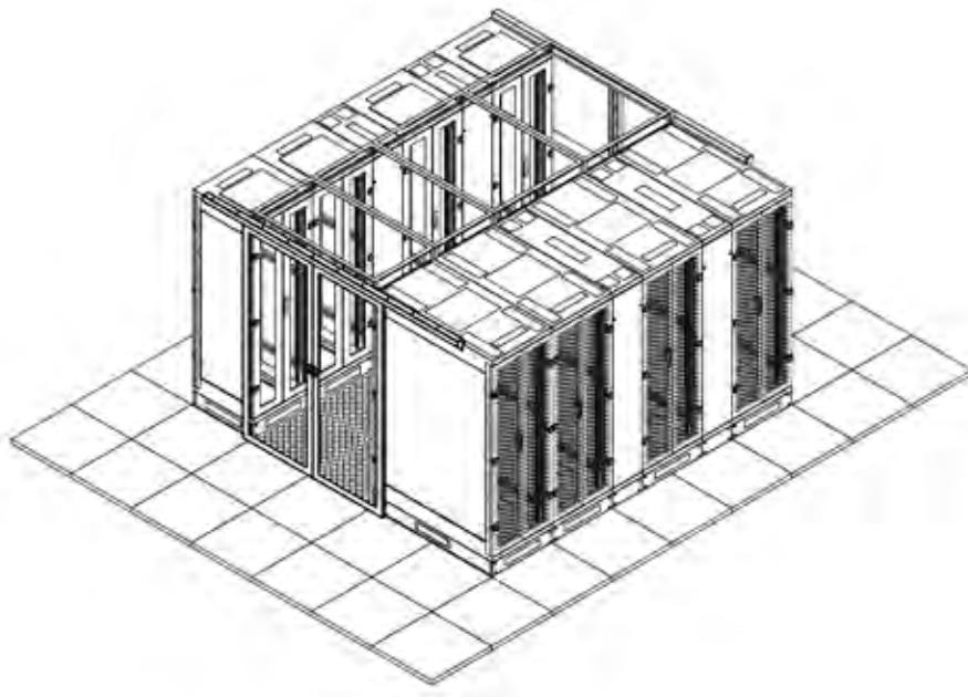
Installed Sliding doors and Roofs
