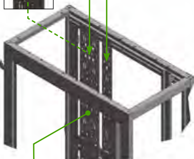
Vertical Lacing/PDU Mounting Panel 3.5" and 7" wide
