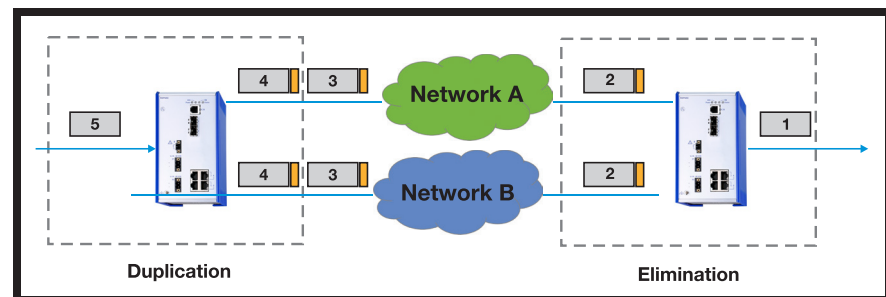
Figure 1. PRP without network failure. Two redundant paths are used simultaneously. Packets duplicated at point 5; duplicates are discarded at point 1.
