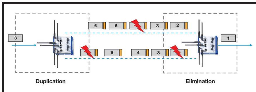
Figure 3. PRP over two WLAN transmission paths: The redundant transmission compensates for packet losses and counterbalances load and interference-related transit time differences.
