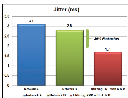
Chart 2. Jitter (ms).
