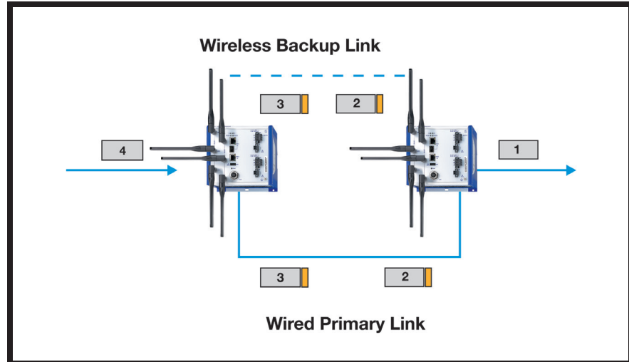
Figure 4. PRP allows both wired and wireless routes to be used as redundant paths, thereby enabling a variety of network topologies. Shown here is a wired path with a wireless backup path.
