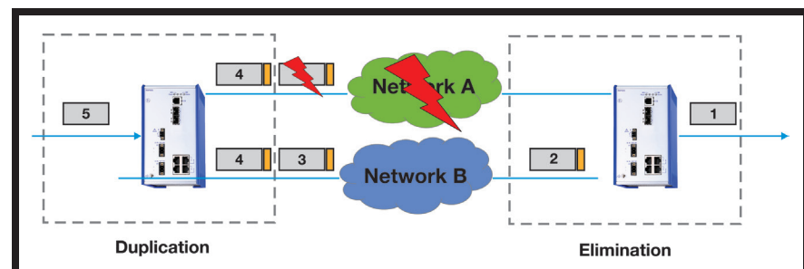
Figure 2. PRP in case of a network failure. Packets from the second network path are used without any resulting switchover times.
