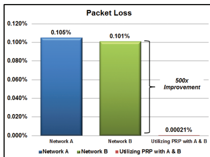
Chart 1. Packet Loss.
