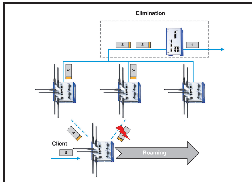
Figure 5. PRP in a WLAN network comprising several access points and a client. Elimination is performed at a central location with a PRP-enabled switch.
