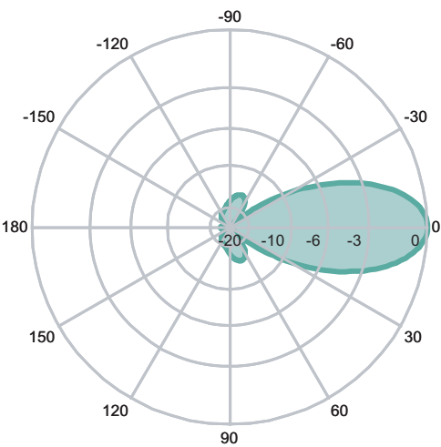
Horizontal 2,400 MHz
