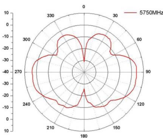
vertical 5750 MHz
