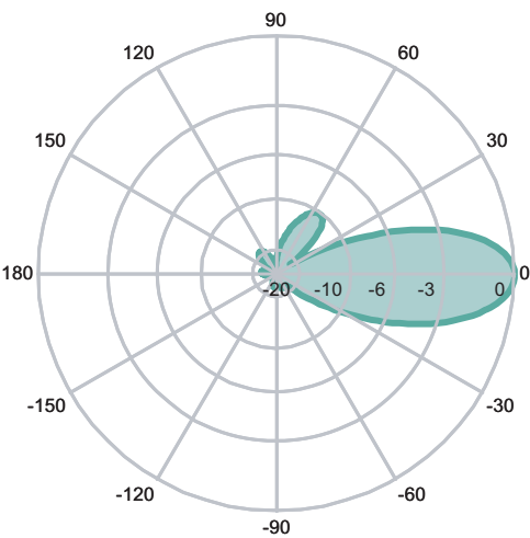
Vertical 2,400 MHz
