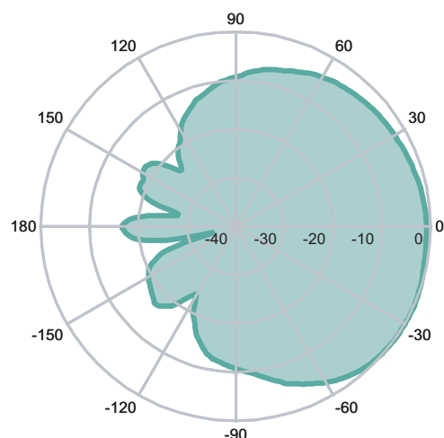
vertical – connection 3
