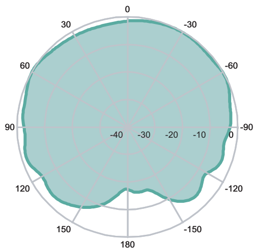
vertical 5470 MHz
