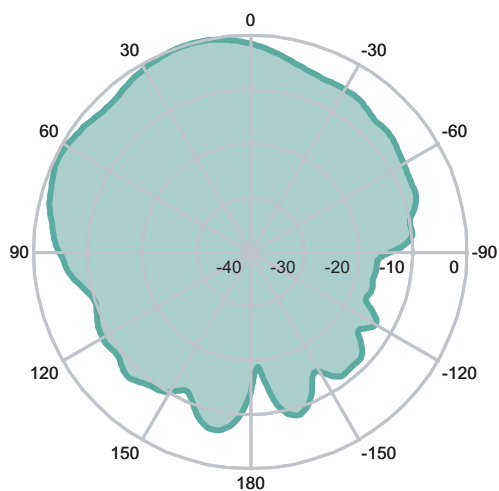
vertical 5470 MHz
